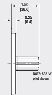
SHAFT CODE 16 3/4"-11T Spline • SAE external involute spline • 3/4" nominal diameter, 11 teeth • 16/32 diametrical pitch • Flat root side fit • Major \phi = 0.729" - 0.734" [18.51-18.64mm] • Minor \phi = 0.597" - 0.608" [15.17-15.45mm]
