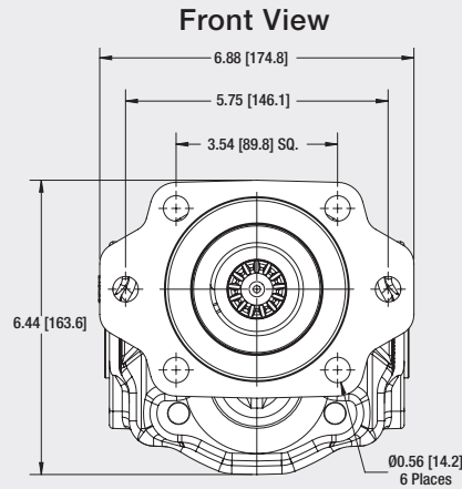
SAE "B" 2/4-Bolt Mounting Flange Shown
