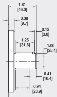
SHAFT CODE 01 SAE "BB" 1.0" Rd. Shaft with 1/4" key NOTE: SAE "B" pilot shown
